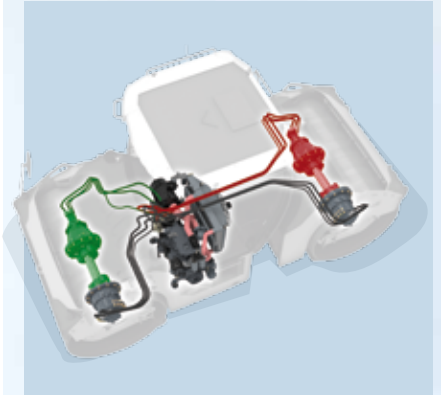
The frequency and amplitude of the front and rear roller drum can be set separately.
