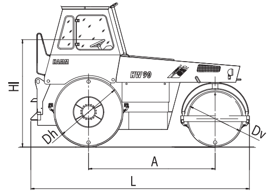
HW 90B/10 - Static three wheel roller 10t HW 90B/12 - Static three wheel roller 12t
