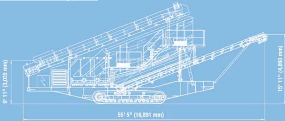
Side view MS 20 D operating position
