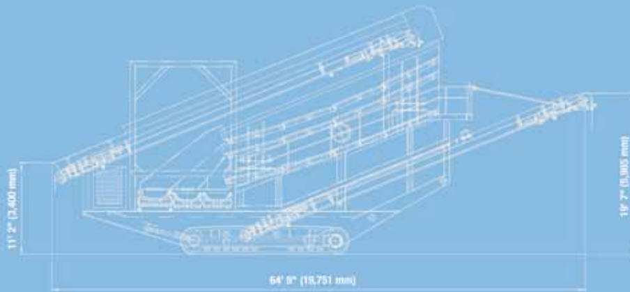
Side view MS 23 D operating position
